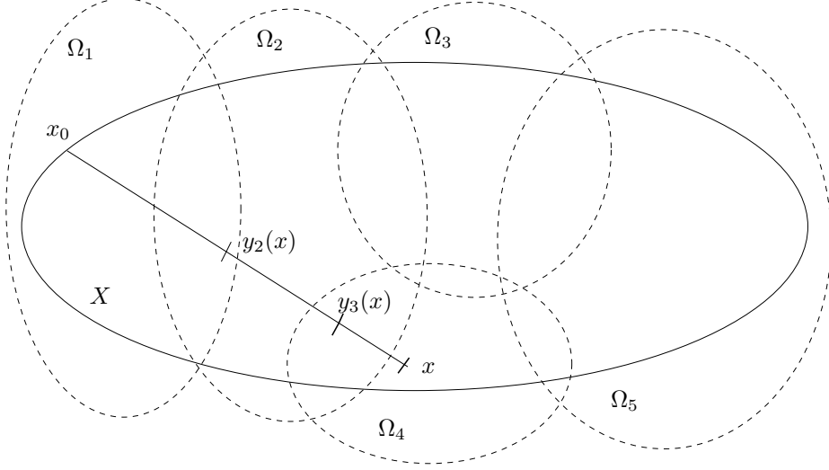
Figure 1: An example of setting for the reconstruction of \sigma at some x \in X . One can see that [x_0, y_2(x)] \subset \Omega_1 , [y_2(x), y_3(x)] \subset \Omega_2 and [y_3(x), x] \subset \Omega_4 . In this case, we have \psi(x, 1) = 1 , \psi(x, 2) = 2 and \psi(x, 3) = 4 .
