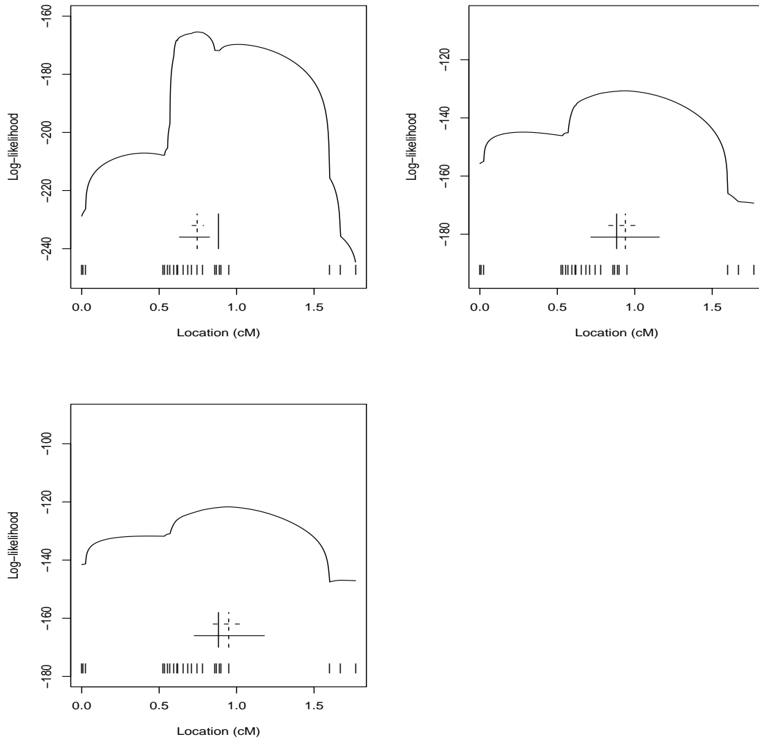
Figure 2: Results of LD mapping for CF haplotype data by the DHS method, where background LD is modeled as Markov( \eta ) with \eta = 0 (upper left), \eta = 1 (upper right), \eta = 2 (lower left). Curve gives log profile likelihood vs. (putative) location x of variant, where x is expressed as distance from D21S1885. The dotted vertical line is the estimated variant location based on affecteds' haplotypes. The unbroken vertical line, unbroken and dotted horizontal lines, and the hash marks have the same meaning as in Figure 1.
