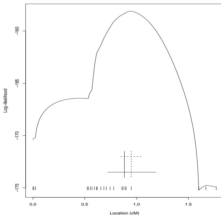
Figure 3: Results of LD mapping for CF genotype data based on a random pairing of affecteds' haplotypes Curve gives log profile likelihood vs. (putative) location x of variant, where x is expressed as distance from D21S1885, and where background LD is modeled as \eta = 2 . The dotted vertical line is estimated location based on affecteds' unphased genotype data. The unbroken vertical line, unbroken and dotted horizontal lines, and the hash marks have the same meaning as in Figure 1.
