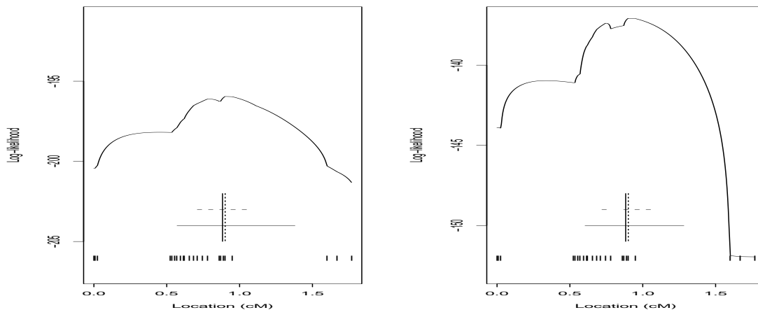
Figure 4: Results of LD mapping for CF genotype data with added heterogeneity (left) with results assuming haplotype data with added heterogeneity shown (right) for comparison. In each case, the curve gives log profile likelihood vs. (putative) location x of variant, where x is expressed as distance from D21S1885, and where background LD is modeled as \eta = 2 . In the top plot, the dotted vertical line is estimated location based on unphased genotype data, while in the bottom plot, the dotted vertical line is estimated location based on haplotype data. The unbroken vertical line, unbroken and dotted horizontal lines, and the hash marks have the same meaning as in Figure 1. The details of the added heterogeneity are given in the text.
